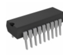
PIC16LC622-04E/P Microchip Technology IC MCU 8BIT 3.5KB OTP 18DIP
