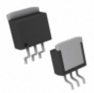
MIC29150-3.3WU-TR Microchip Technology IC REG LDO 3.3V 1.5A TO263-3
