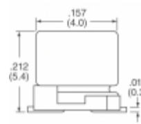
AVRF106M25B12T-F Cornell Dubilier Electronics (CDE) CAP ALUM 10UF 20% 25V SMD
