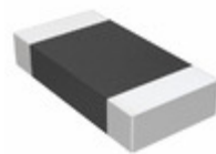
CC1206MRX7R9BB473 Yageo CAP CER 0.047UF 50V X7R 1206
