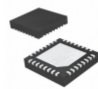
DSPIC33EP128MC202T-I/MM Microchip Technology IC MCU 16BIT 128KB FLASH 28QFN
