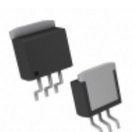
LD29300D2M18 STMicroelectronics IC REG LDO 1.8V 3A D2PAK/A
