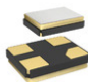
FA-20H 32.0000MF20X-K0 EPSON CRYSTAL 32.00 MHZ 10.0PF SMD
