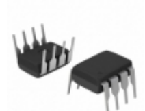
AT25320A-10PI-2.7 Microchip Technology IC EEPROM 32KBIT 20MHZ 8DIP
