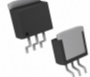
MCP1827S-3002E/EB Microchip Technology IC REG LDO 3V 1.5A 3DDPAK
