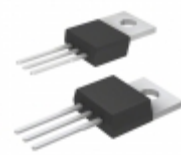
MCP1827S-1802E/AB Microchip Technology IC REG LDO 1.8V 1.5A TO220-3
