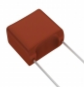
ECW-F2W225KA Panasonic Electronic Components CAP FILM 2.2UF 10% 450VDC RADIAL
