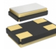
FA-238 27.0000MB-AJ3 EPSON CRYSTAL 27.00 MHZ 8.0PF SMD
