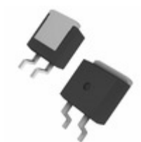
IXGA120N30TC IXYS IGBT 300V 120A 250W TO263AA
