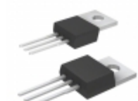
IXFP26N50P3 IXYS MOSFET N-CH 500V 26A TO-220
