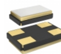
FA-238 40.0000MB-C0 EPSON CRYSTAL 40.00 MHZ 18.0PF SMD
