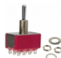
7401SCWCGE C&K SWITCH TOGGLE 4PDT 5A 120V
