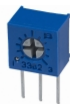
3362M-1-501ALF Bourns, Inc. TRIMMER 500 OHM 0.5W PC PIN SIDE
