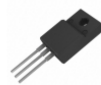
AOTF2916L Alpha & Omega Semiconductor Inc. MOSFET N-CH 100V 5A TO220F
