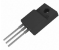
AOTF2918L Alpha & Omega Semiconductor Inc. MOSFET N-CH 100V 58A TO220F
