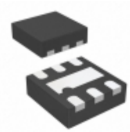
MIC5364-3.3YMT-TR Microchip Technology IC REG LDO 3.3V 0.3A 6TMLF
