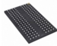
IS49NLC36800-25BLI ISSI, Integrated Silicon Solution Inc IC DRAM 288MBIT 400MHZ 144BGA
