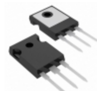
VS-60APF02PBF Electro-Films (EFI) / Vishay DIODE GEN PURP 200V 60A TO247AC
