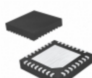
PIC16F1827T-I/MV Microchip Technology IC MCU 8BIT 7KB FLASH 28UQFN
