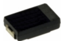
EEF-CX1D470R Panasonic Electronic Components CAP ALUM POLY 47UF 20% 20V SMD
