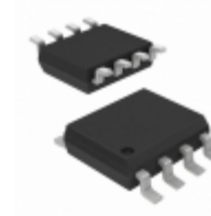
IRF7233TRPBF Infineon Technologies MOSFET P-CH 12V 9.5A 8-SOIC
