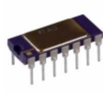
AD536AKDZ Analog Devices Inc. IC TRUE RMS/DC CONV 14-CDIP
