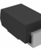
SMAJ160A-E3/5A Electro-Films (EFI) / Vishay TVS DIODE 160V 259V DO214AC
