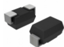
SMAJ160A Bourns Inc. TVS DIODE 160VWM 259VC DO214AC
