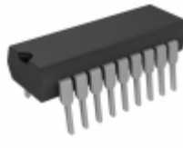
PIC24HJ12GP201-I/P Microchip Technology IC MCU 16BIT 12KB FLASH 18DIP
