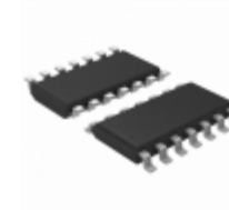
IX2B11S7T/R IXYS IC DRVR HALF BRIDGE GATE 14-SOIC
