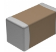
CDR32BP1R0BCZRAT Vishay Vitramon CAP CER 1PF 100V BP 1206
