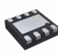
ADT7408CCPZ-REEL Analog Devices Inc. SENSOR TEMP I2C/SMBUS 8LFCSP
