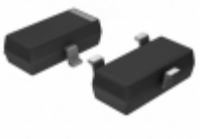
S-1206B25-M3T1G SII Semiconductor Corporation IC REG LINEAR 2.5V 0.25A SOT23-3
