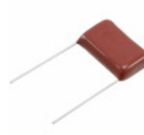
ECQ-E6474KFB Panasonic Electronic Components CAP FILM 0.47UF 10% 630VDC RAD
