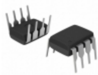
AT25640A-10PU-1.8 Microchip Technology IC EEPROM 64KBIT 20MHZ 8DIP
