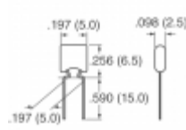
B37987F1154K051 EPCOS (TDK) CAP CER 0.15UF 100V X7R RADIAL
