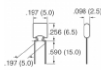
B37987F1104K054 EPCOS (TDK) CAP CER 0.1UF 100V X7R RADIAL
