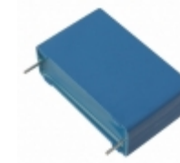
B32676G1565K EPCOS (TDK) CAP FILM 5.6UF 10% 750VDC RADIAL
