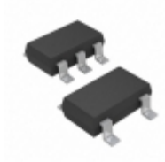
MIC5259-1.8YD5-TR Microchip Technology IC REG LDO 1.8V 0.3A TSOT23-5
