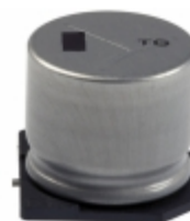
EEV-TG1C222M Panasonic Electronic Components CAP ALUM 2200UF 20% 16V SMD
