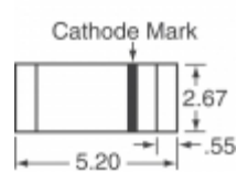
DL4754A-TP Micro Commercial Co DIODE ZENER 39V 1W MELF
