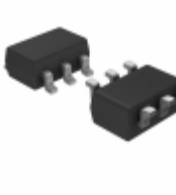
ADA4897-1SRJZ-EPR7 Analog Devices Inc. IC OPAMP GP 230MHZ RRO SOT23-6
