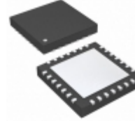
PIC18F25Q10T-I/ML Micrel / Microchip Technology 32KB FLASH, 2KB RAM, 256B EEPROM
