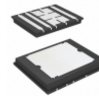
SIE860DF-T1-GE3 Vishay Siliconix MOSFET N-CH 30V 60A POLARPAK
