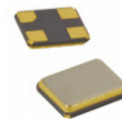
NX3225SA-16.000000MHZ-B3 NDK America, Inc. CRYSTAL 16.0000MHZ 7.2PF SMD
