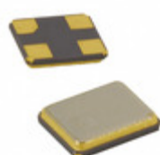
NX3225SA-14.31818MHZ-STD-CSR-1 NDK America, Inc. CRYSTAL 14.31818MHZ 8PF SMD
