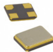
NX3225SA-16.000000MHZ-T1 NDK America, Inc. CRYSTAL 16.0000MHZ 10PF SMD
