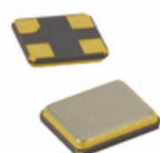
NX3225SA-13M-STD-CSR-6 NDK America, Inc. CRYSTAL 13.0000MHZ 8PF SMD
