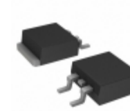
HUF75842S3ST AMI Semiconductor / ON Semiconductor MOSFET N-CH 150V 43A D2PAK
