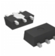
XC6222B331PR-G Torex Semiconductor Ltd. IC REG LDO 3.3V 0.7A SOT89-5
