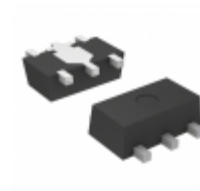
XC6222B28BPR-G Torex Semiconductor Ltd. IC REG LDO 2.85V 0.7A SOT89-5
