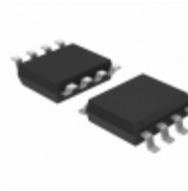
24LC08B/SN Microchip Technology IC EEPROM 8KBIT 400KHZ 8SOIC
