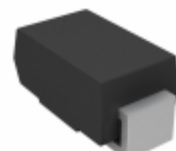
TPSMA7.5AHE3/61T Vishay Semiconductor Diodes Division TVS DIODE 6.4VWM 11.3VC SMA
