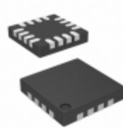
CY8C20234-12LKXI Cypress Semiconductor Corp IC MCU 8BIT 8KB FLASH 16QFN
