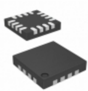
CY8C20234-12LKXIT Cypress Semiconductor Corp IC MCU 8BIT 8KB FLASH 16QFN
