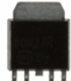
AN80M27RSP Panasonic Electronic Components IC REG LDO 2.7V 0.5A SP4SUA
