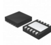
MCP4232-104E/MF Microchip Technology IC POT DGTL DUAL 100K RHEO 10DFN
