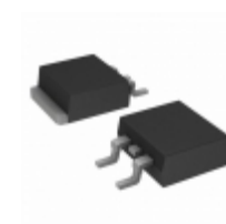
IRF2805SPBF Infineon Technologies MOSFET N-CH 55V 135A D2PAK
