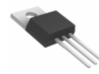
D44H8 Fairchild/ON Semiconductor TRANS NPN 60V 8A TO-220
